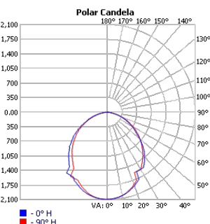
TECHOLED-ASC-D-31-HI-30
