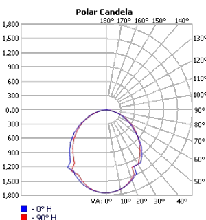
TECHOLED-ASC-D-23-HI-30
