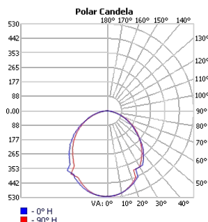
TECHOLED-ASC-D-14-ME-30
