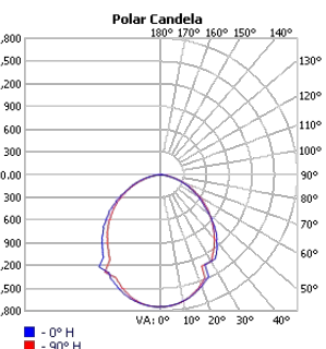
TECHOLED-ASC-D-31-ME-30
