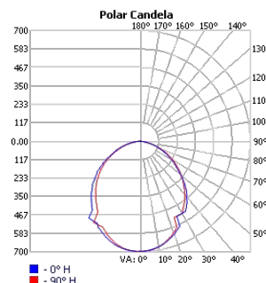
TECHOLED-ASC-D-14-HI-30
