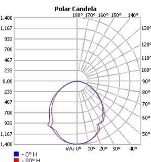
TECHOLED-ASC-D-31-LO-30
