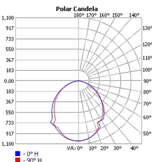
TECHOLED-ASC-D-17-HI-30
