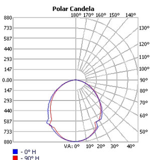
TECHOLED-ASC-D-17-ME-30
