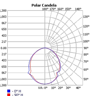
TECHOLED-ASC-D-23-ME-30
