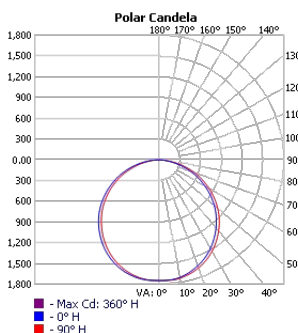
TECHOLED-ASY-D-42-LO-30
