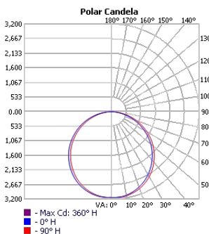
TECHOLED-ASY-D-63-LO-30
