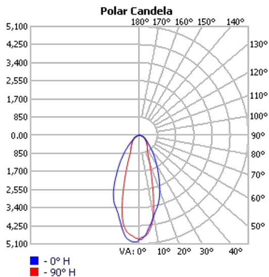
TECHOLED-BX-1LH-D-8-ME-30
