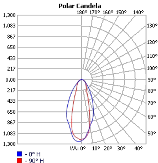
TECHOLED-BX-1LH-D-2-ME-30
