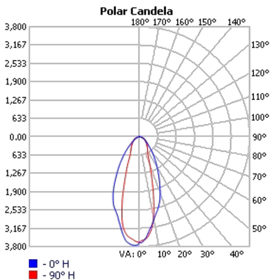
TECHOLED-BX-1LH-D-6-ME-30
