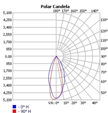
TECHOLED-BX-3S-D-6-ME-30
