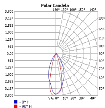
TECHOLED-BX-3S-D-4-ME-30
