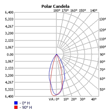
TECHOLED-BX-3S-D-8-ME-30
