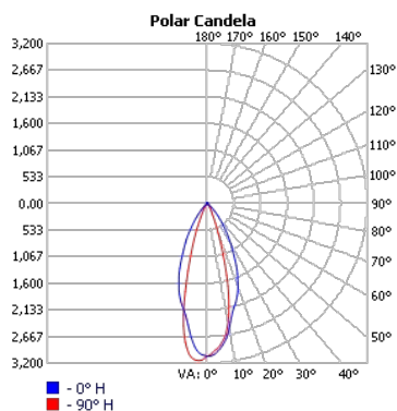
TECHOLED-BX-3S-D-2-ME-30
