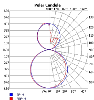
TECHOLED-BX-4-DI-2-ME-30
