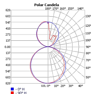
TECHOLED-BX-4-DI-2-HI-30
