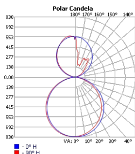
TECHOLED-BX-4-DI-4-LO-30
