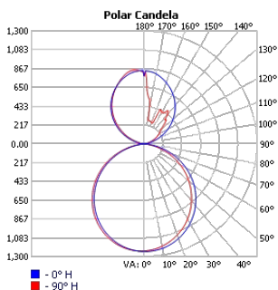
TECHOLED-BX-4-DI-6-LO-30
