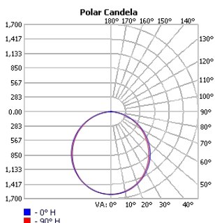
TECHOLED-BX-4-D-8-LO-30
