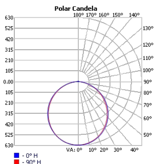
TECHOLED-BX-4-D-2-ME-30
