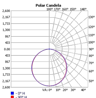
TECHOLED-BX-4-D-8-ME-30
