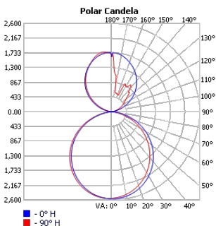
TECHOLED-BX-4-DI-8-ME-30
