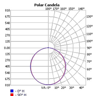
TECHOLED-BX-4-D-2-HI-30
