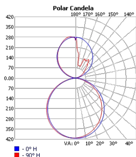
TECHOLED-BX-4-DI-2-LO-30
