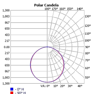
TECHOLED-BX-4-D-4-ME-30
