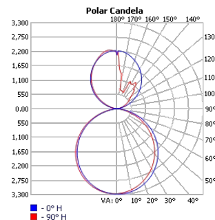
TECHOLED-BX-4-DI-8-HI-30
