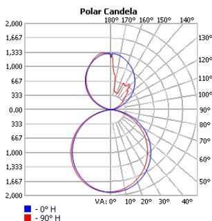
TECHOLED-BX-4-DI-6-ME-30
