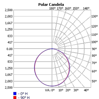
TECHOLED-BX-4-D-6-HI-30
