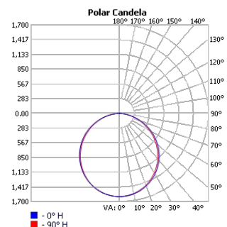
TECHOLED-BX-4-D-4-HI-30
