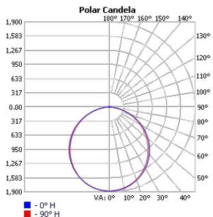
TECHOLED-BX-4-D-6-ME-30
