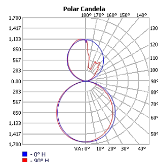
TECHOLED-BX-4-DI-4-HI-30
