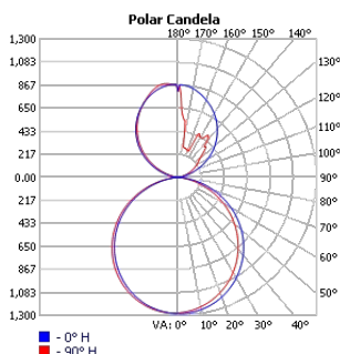
TECHOLED-BX-4-DI-4-ME-30
