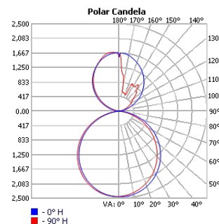
TECHOLED-BX-4-DI-6-HI-30
