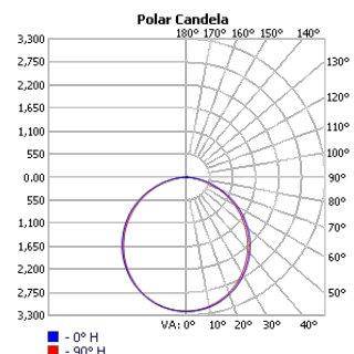
TECHOLED-BX-4-D-8-HI-30
