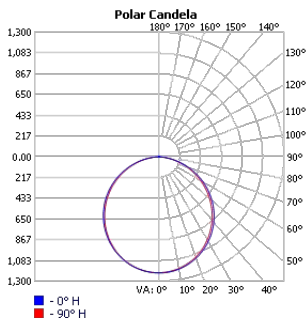
TECHOLED-BX-4-D-6-LO-30
