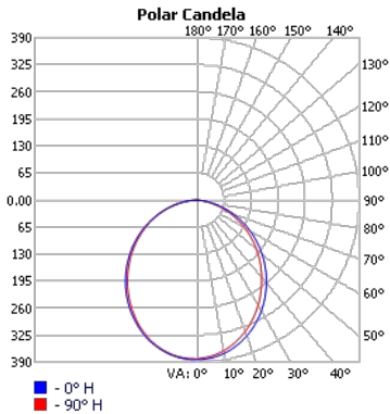
TECHOLED-BX-CURV-R-D-C-ME-30
