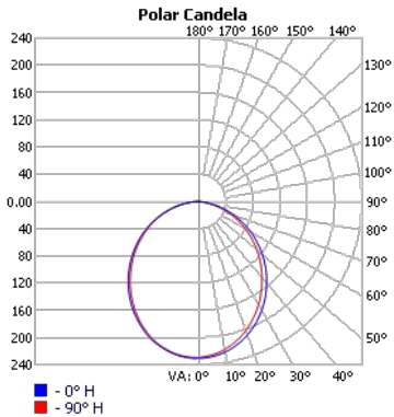
TECHOLED-BX-CURV-R-D-C-LO-30
