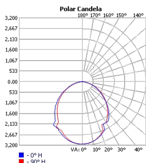
TECHOLED-HALO-D-95-LO-30
