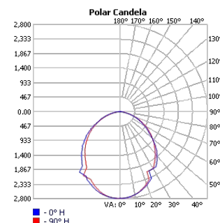
TECHOLED-HALO-D-35-HI-30
