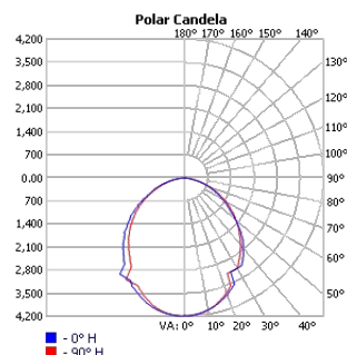
TECHOLED-HALO-D-78-ME-30
