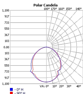
TECHOLED-HALO-D-35-LO-30
