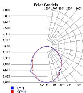
TECHOLED-HALO-D-196-LO-30
