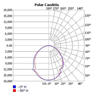
TECHOLED-HALO-D-196-HI-30
