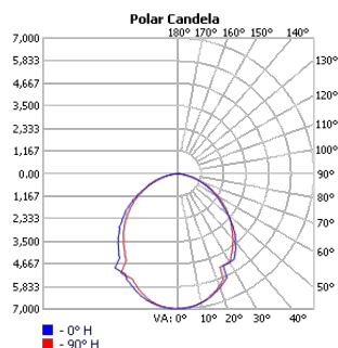
TECHOLED-HALO-D-118-ME-30
