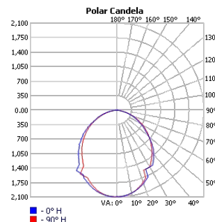
TECHOLED-HALO-D-23-HI-30
