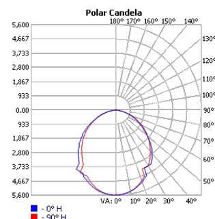
TECHOLED-HALO-D-59-HI-30
