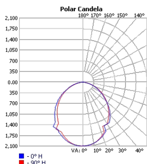
TECHOLED-HALO-D-78-LO-30
