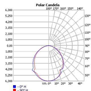
TECHOLED-HALO-D-78-HI-30
