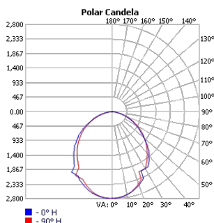
TECHOLED-HALO-D-47-ME-30
