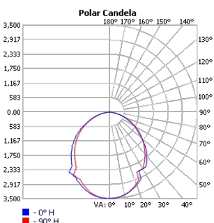
TECHOLED-HALO-D-59-ME-30
