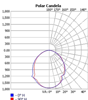
TECHOLED-HALO-D-59-LO-30
