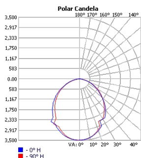
TECHOLED-HALO-D-118-LO-30
