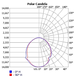
TECHOLED-HALO-D-196-ME-30
