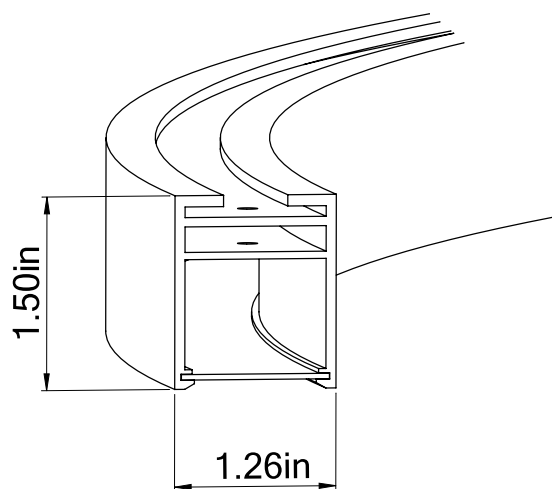
Cross Section
