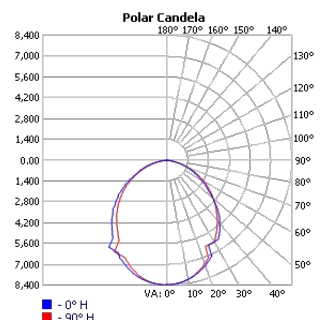
TECHOLED-HALO-D-95-HI-30
