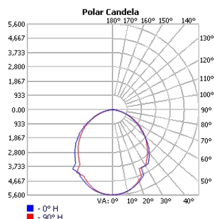
TECHOLED-HALO-D-95-ME-30
