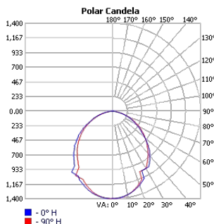
TECHOLED-HALO-D-23-ME-30
