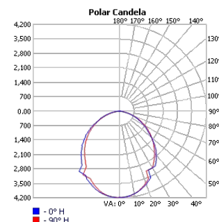
TECHOLED-HALO-D-47-HI-30
