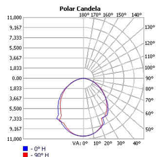
TECHOLED-HALO-D-118-HI-30
