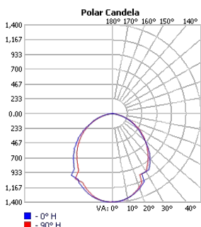
TECHOLED-HALO-D-47-LO-30
