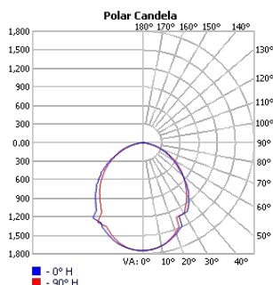
TECHOLED-HALO-D-35-ME-30
