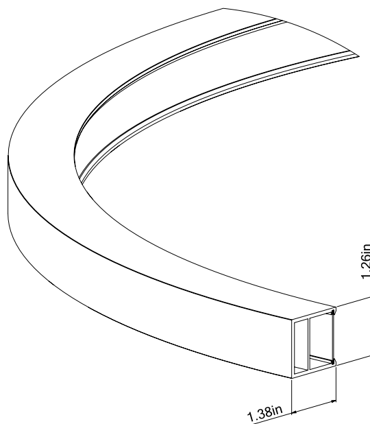
Cross Section
