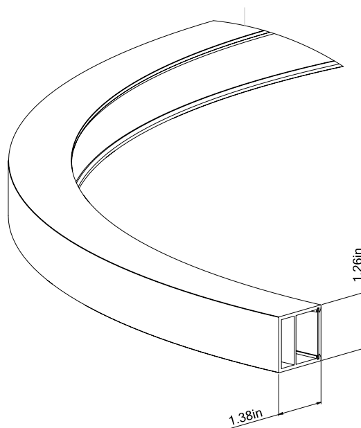
Cross Section
