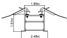
LED Light Cross Section
