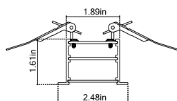
LED Light Section
