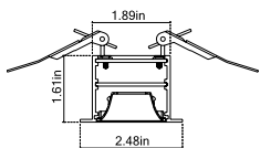
Louver Cross Section
