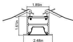
Louvre Section
