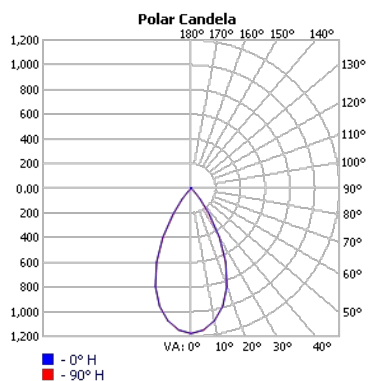
TECHOLED-HALO-L-D
