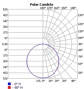
TECHOLED-HALO-L-D
