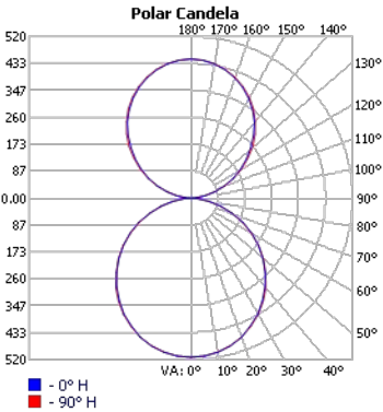
TECHOLED-HALO-L-DI
