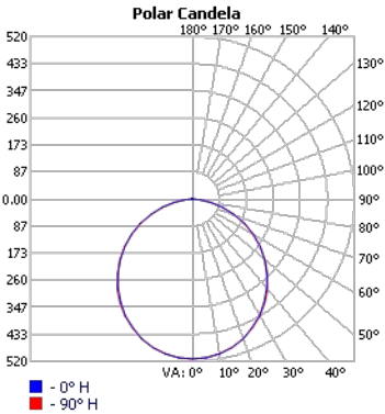
TECHOLED-HALO-L-D
