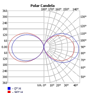
TECHOLED-HALO-O-35-ME-30
