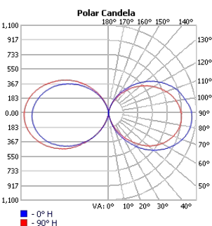
TECHOLED-HALO-O-59-HI-30
