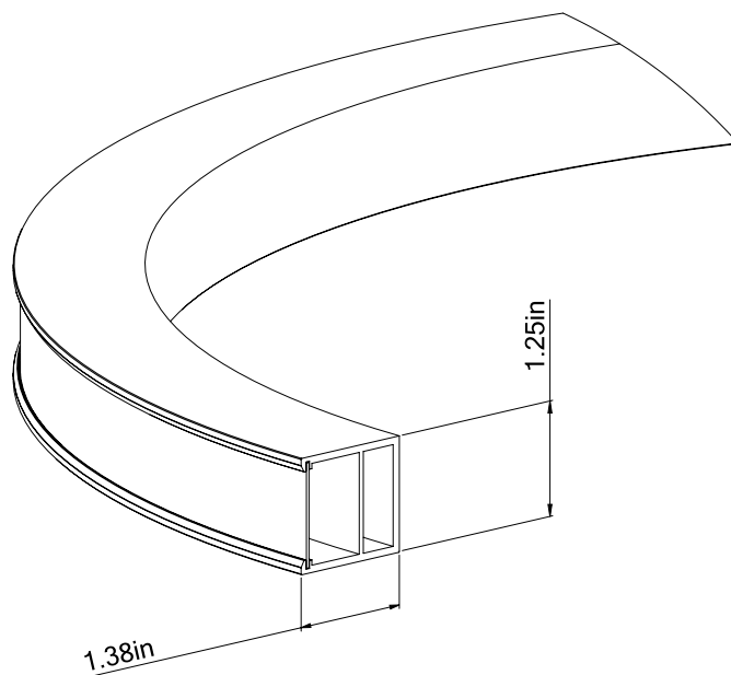
Cross Section
