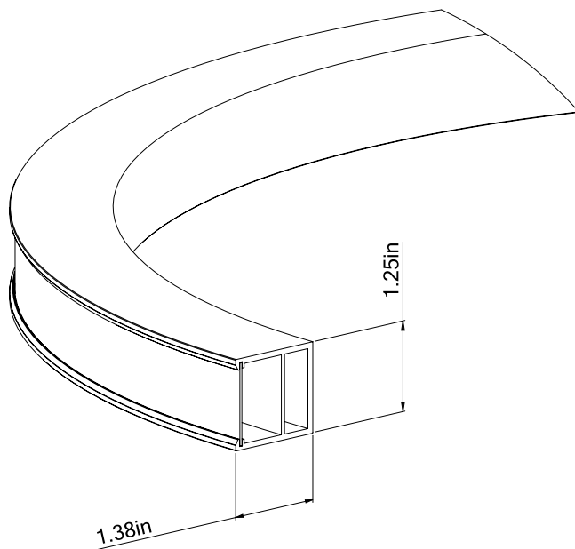
Cross Section
