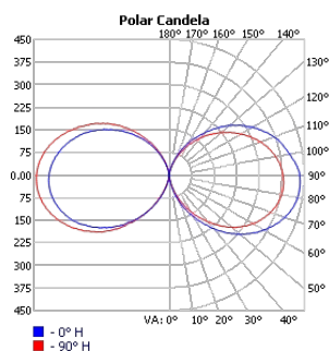
TECHOLED-HALO-O-59-LO-30
