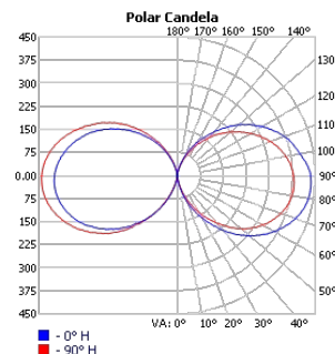
TECHOLED-HALO-O-23-HI-30
