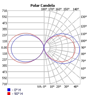
TECHOLED-HALO-O-59-ME-30
