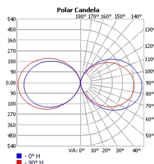
TECHOLED-HALO-O-35-HI-30
