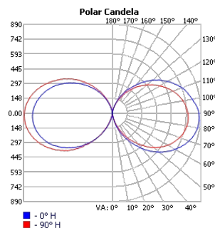
TECHOLED-HALO-O-47-HI-30
