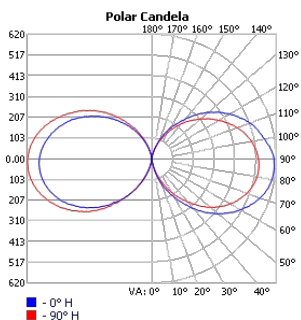
TECHOLED-HALO-O-47-ME-30
