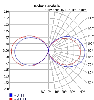
TECHOLED-HALO-O-35-LO-30
