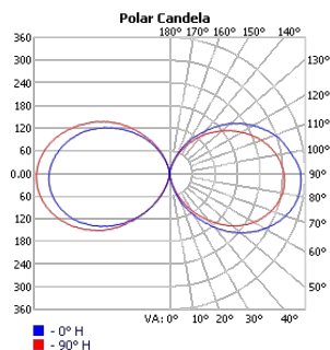
TECHOLED-HALO-O-47-LO-30
