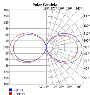
TECHOLED-HALO-O-23-LO-30
