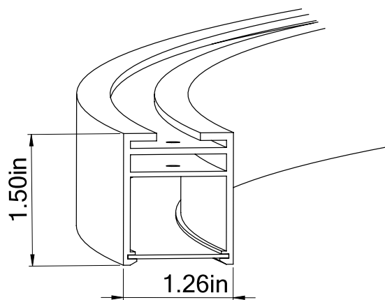
Cross Section
